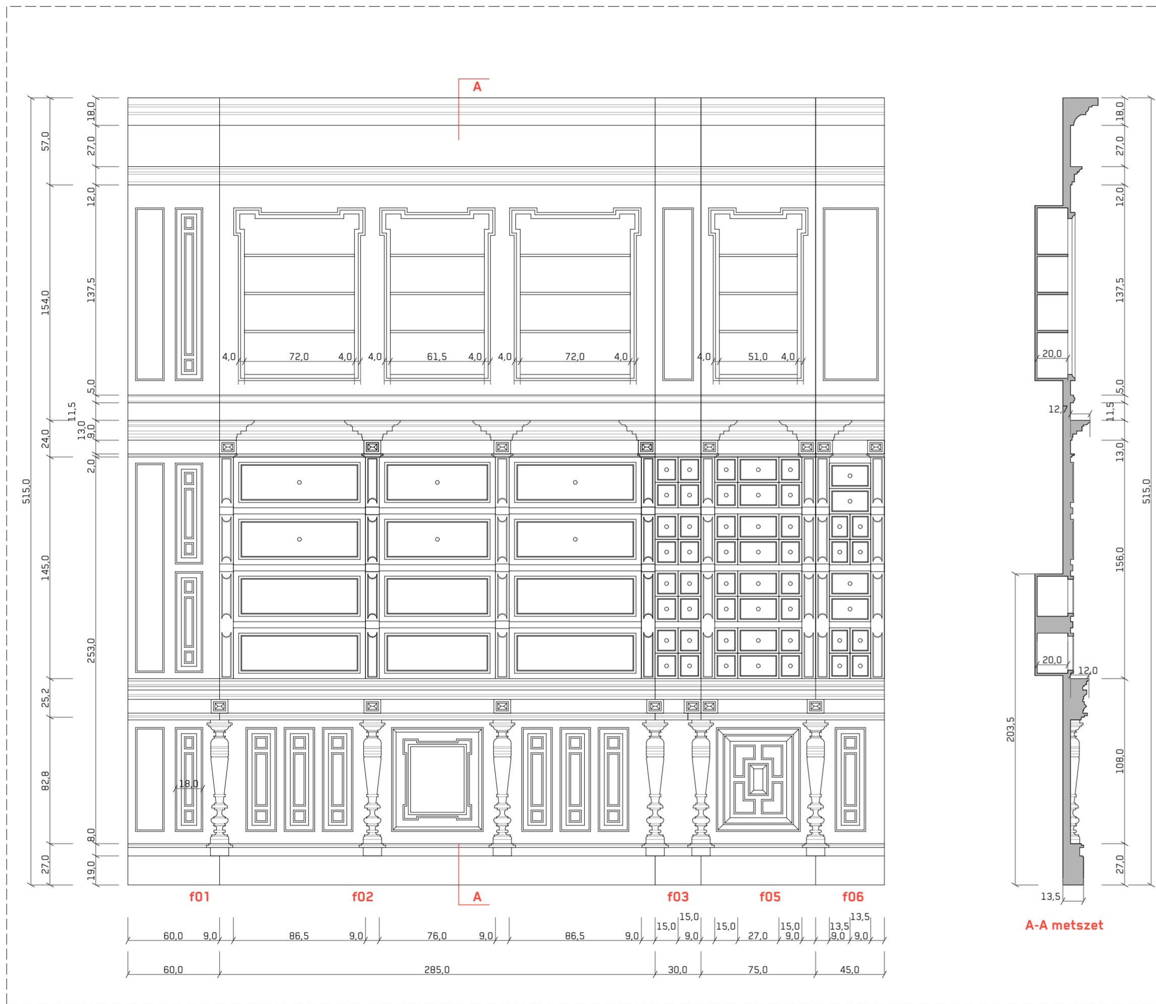
BAL PORTAL FAL 1:25
